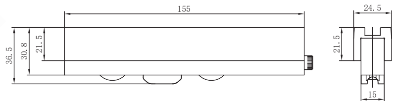
Bánh xe Xingfa 2 bánh
